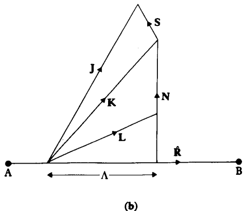
10.14 Angular momentum vectors in Hund's cases (a) and (b).
